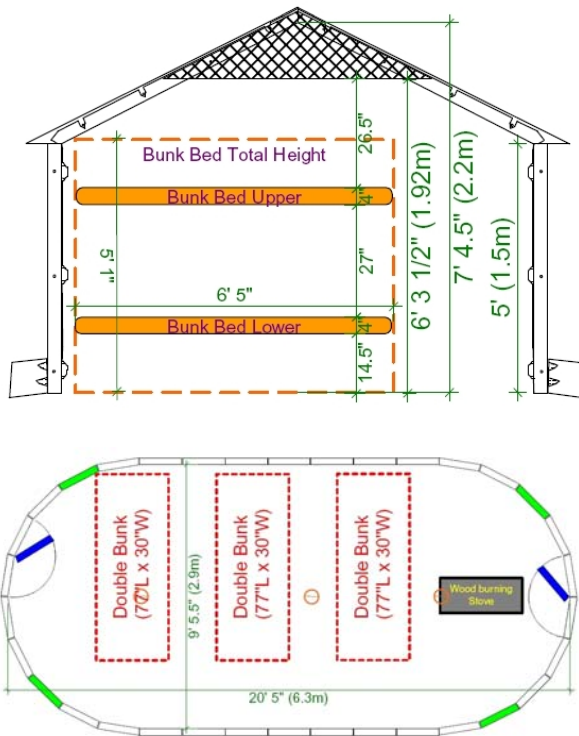
SegYurt-7 with bunk beds
